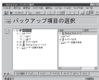
BackupExec
