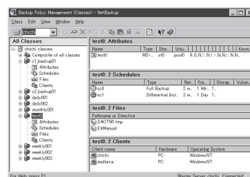
NetBackup
