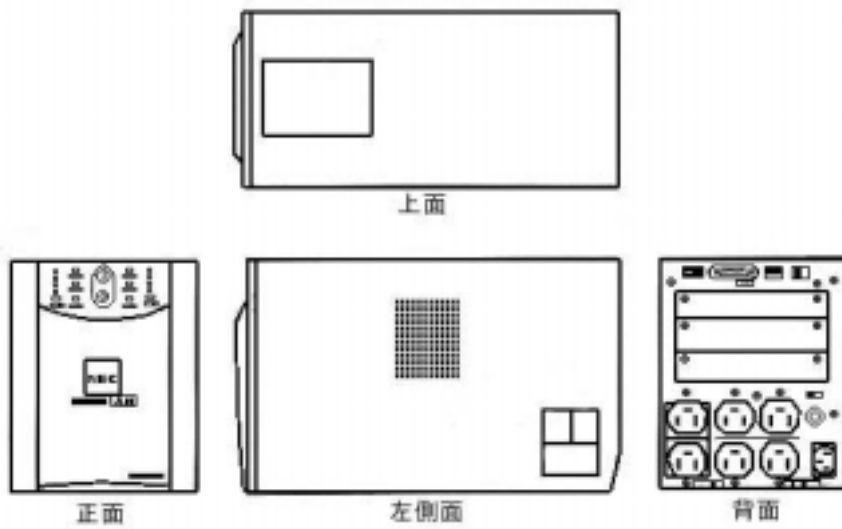
(N8580-28AC,29AC) 170mm(W)×570mm(D)×219mm(H)
