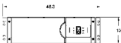
(N8542-11) 483mm(W)×635mm(D)×130mm(H)
