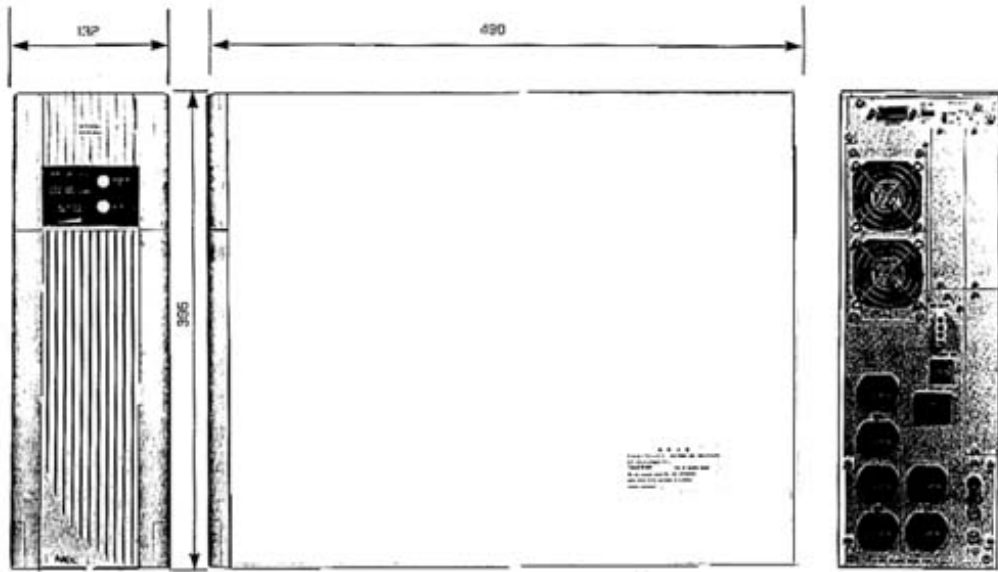
(N8580-27A) 132mm(W)×490mm(D)×395mm(H)
